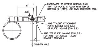
TOP ACCESS "TALON" BRACKET ASSEMBLY NTS
